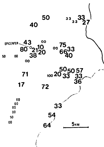
Fig. 6. Distribution of people who heard the sound just before the earthquake. Ratio of the persons perceived the sound and the all answers is indicated by numbers in percentage.
