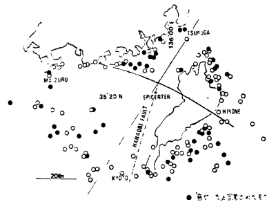
Fig. 8. Distribution of persons who heard the sound before the earthquake in B region. Solid circles mean the persons who heard the sound.
