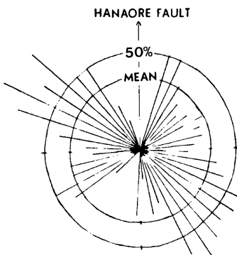
Fig. 11. Directionality of vertical motions.
