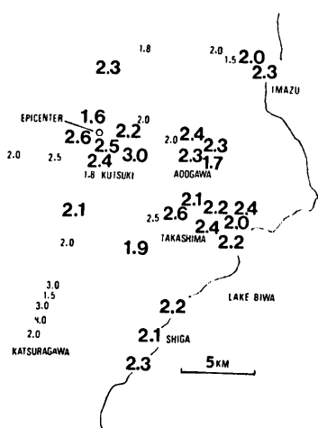
Fig. 5. Distribution of seismic intensity near the epicenter. Large numerals means the answers were over 5 and small one under 4 answers.
