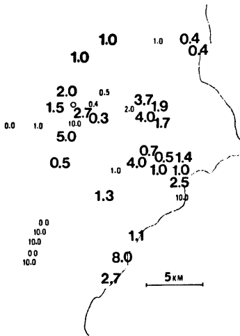
Fig. 7. Distribution of people who felt vertical motion. Numerals indicate ratio of the number of people who felt the vertical motion and the number of persons who felt transverse motion.
