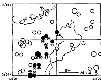
Fig. 2. Locations of epicenters of earthquakes ( M > 2 ) occurred between 1926 and Jul. 1979 near around Hanaore Fault. Numbers indicate time of the earthquakes. Solid circles show the earthquakes along near Hanaore Fault. The double circle indicates the earthquake occurred 16, Oct., 1979.
