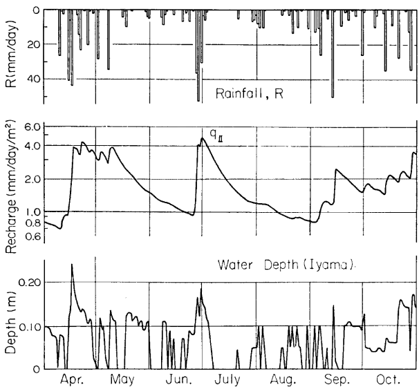
Fig. 13. Hydrographs of recharge from ground surface and water level at Iyama station in the River Kusano.
