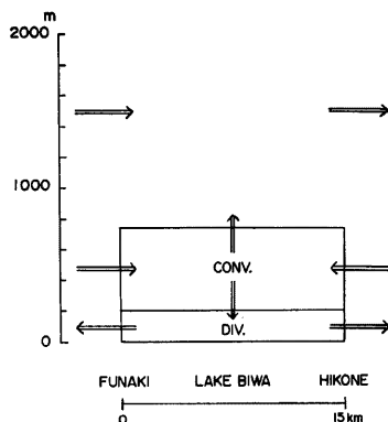
Fig. 10. Vertical circulation of the lake breeze over the northern part of the Lake Biwa at 1200 JST 9 Aug. 1978.
