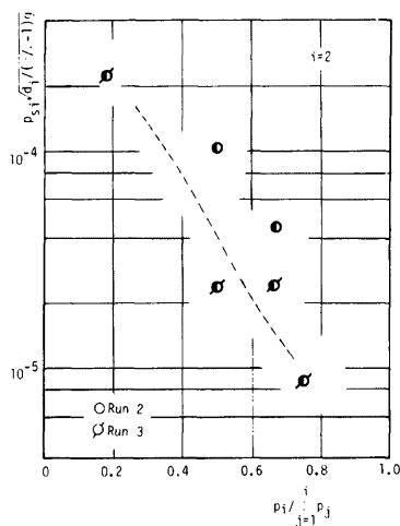
Fig. 21. The relationship between p_{si} and \sqrt{d_i / (\sigma / \rho - 1) g} and \sum_{j=1}^i p_j .
