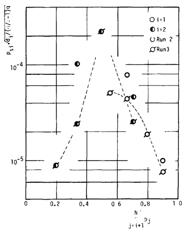
Fig. 20. The relationship between p_{si} and \sqrt{d_i / (\sigma / \rho - 1) g} and \sum_{j=i+1}^N p_j .
