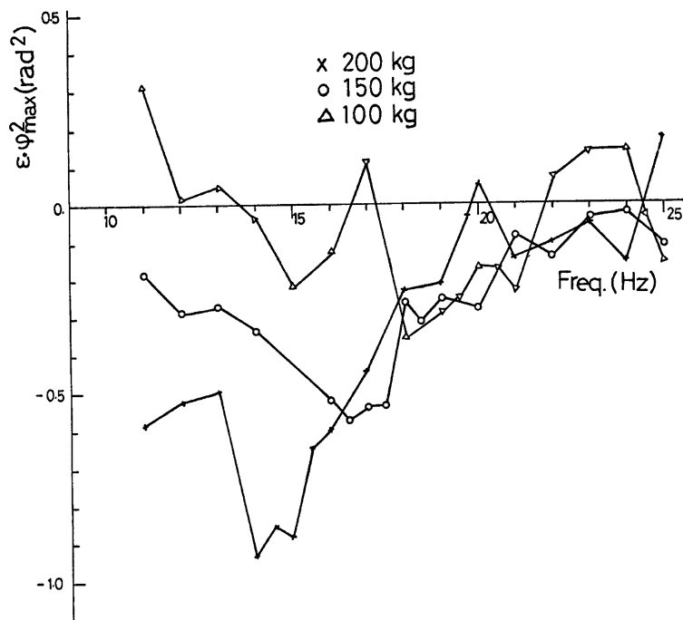
Fig. 20. \varepsilon \cdot \phi_{\max}^2 given by eq.(19).
