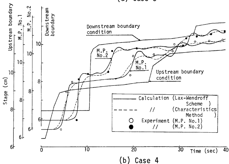
Fig. 6. Comparative representations of unsteady flows in experimental flume -Surge- (a) case 3, (b) case 4.
