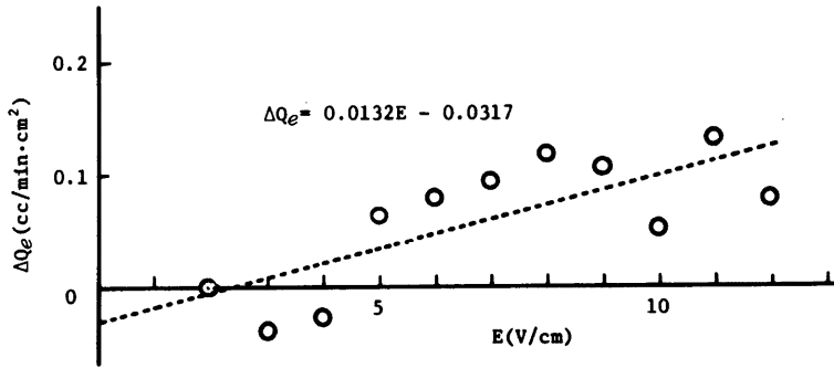
Fig. 2. Water flux \Delta Q_e as a function of E when dh=5 (cm), sand core length is 14 (cm), NaCl concentration is 0.5%, sand particle size is 500\sim 1000 ( \mu ) and porosity is 0.40.
