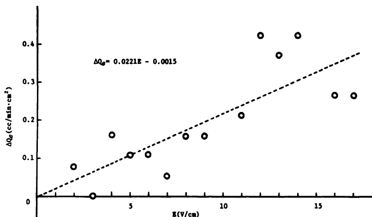
Fig. 4. Water flux \Delta Q_e as a function of E when \Delta h=5 (cm), sand core length is 14 (cm), NaCl concentration is 0.25%, sand particle size is 500~1000( \mu ) and porosity is 0.40.
