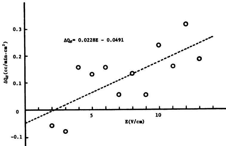
Fig. 3. Water flux \Delta Q_e as a function of E when dh=5 (cm), sand core length is 7 (cm), NaCl concentration is 0.5%, sand particle size is 250\sim 500 ( \mu ) and porosity is 0.44.
