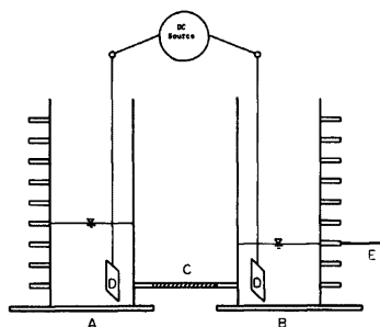
Fig. 1. Profile of the experimental apparatus.
