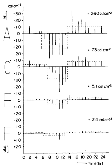
Fig. 11. Variations of releasing and absorbing heat quantity at each time in invariable layer.
