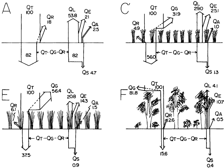
Fig. 10. Relation between surface ground condition and solar radiation.
