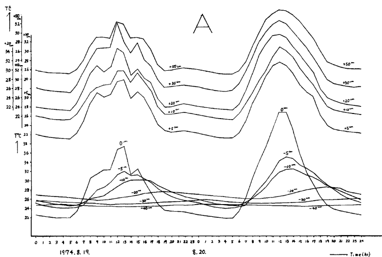
Fig. 4. Diurnal variations of air and underground temperature at the bare land (1974. 8. 19-20).
