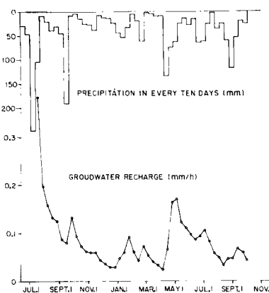
Fig. 7 Ten days' sums of precipitation and groundwater recharge.
