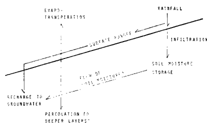
Fig. 11 Schematic representation of the components of hydrologic cycle on mountain slope.
