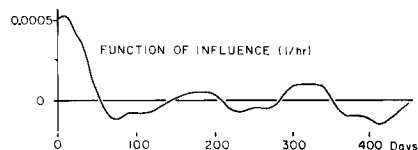
Fig. 8 Function of influence calculated according to the data shown in Fig. 7.
