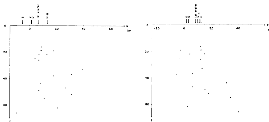
Fig. 3(B),(C) Hypocentres projected to the vertical planes.
