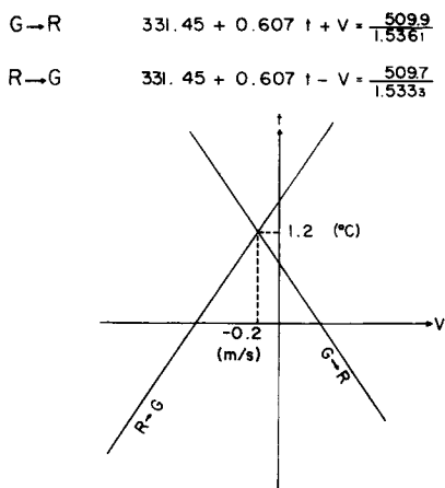
Fig. 3. Sound velocity, temperature and effect of wind.
