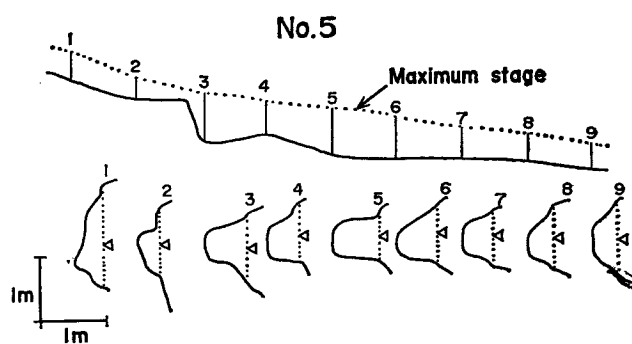
Fig 9 Cross-section and profile for the highest water level of the 1971, 6, 11th flood.
