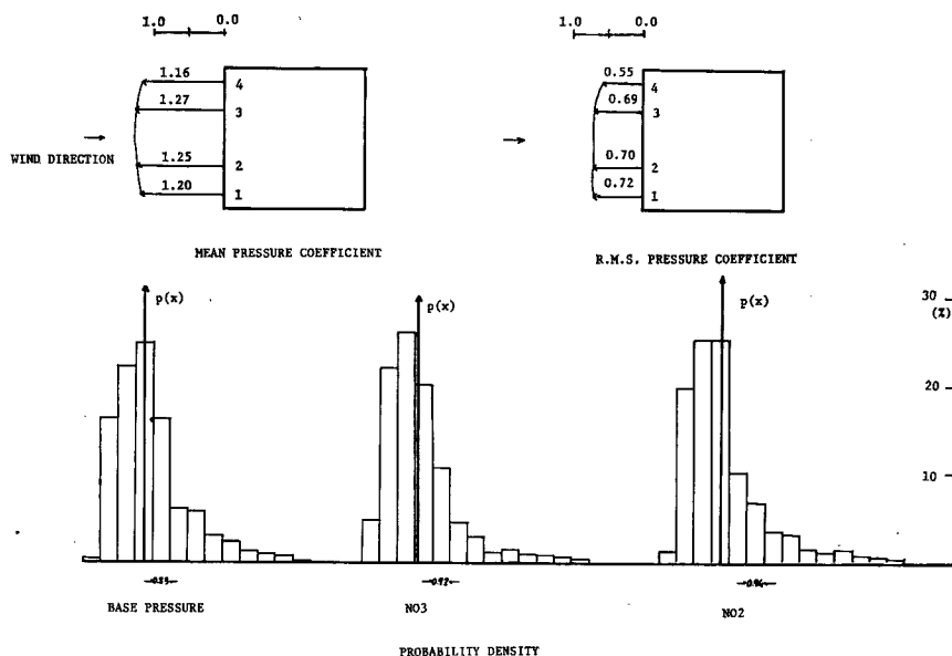
Fig. 3 Pressure coefficients and probability density of the fluctuating pressure.
