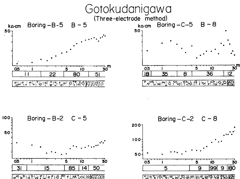
Fig. 6 Relation among \rho - a curve, electric resistivity value and geological phenomena.
