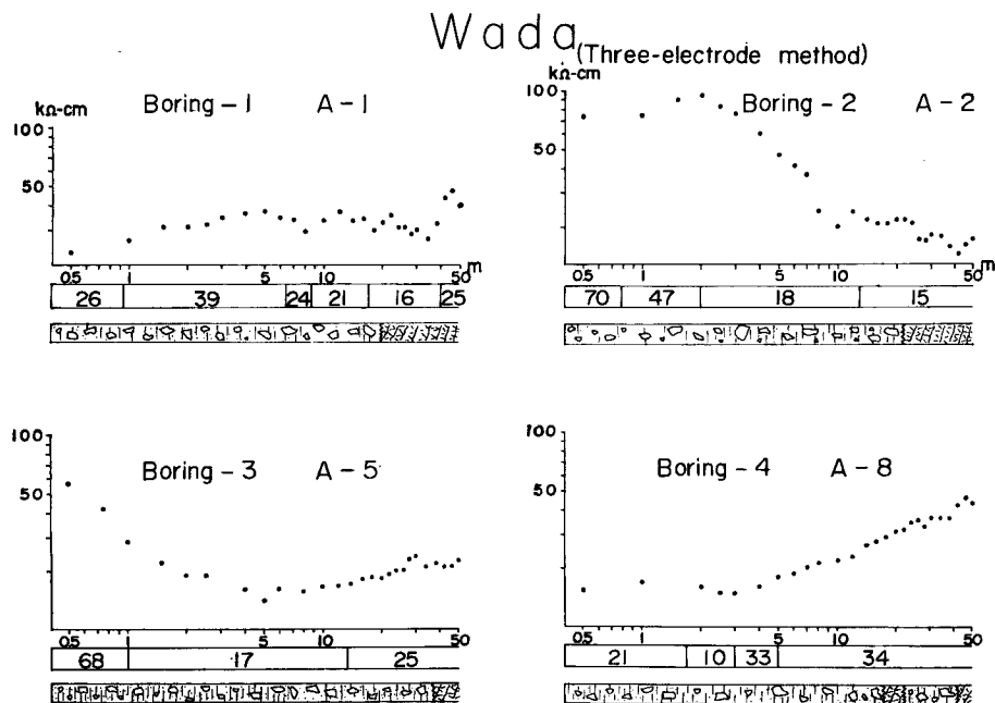
Fig. 7 Relation among \rho - a curve, electric resistivity value and geological phenomena.
