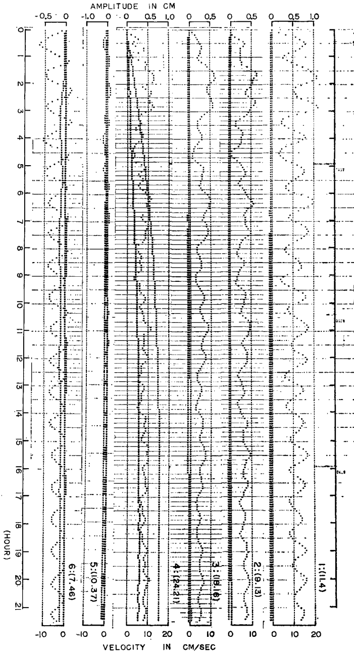
Fig. 4(a) Computed variations of vertical displacement of water surface (mark*), x- and y- component of velocity (mark \square and \triangleright ).
