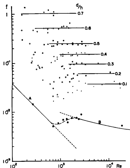
Fig. 28 Friction factor for the wire net.
