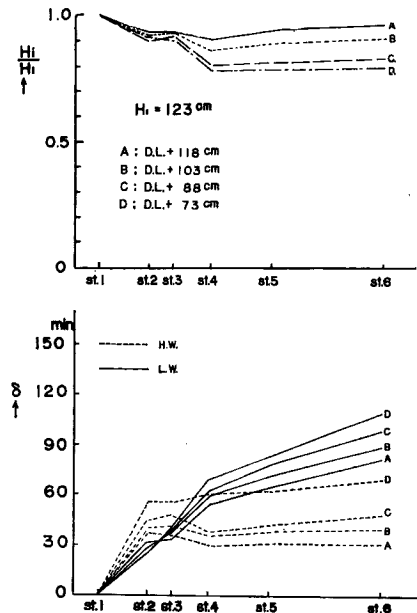
Fig. 22 Effect of mean sea level on the ratio of amplitude H_i/H_1 and phase lag \delta . (dredged state, H_i=123 cm)
