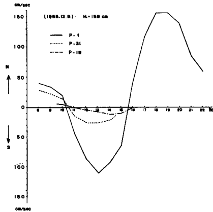
Fig. 5 Time change of velocity of tidal current. (prototype)
