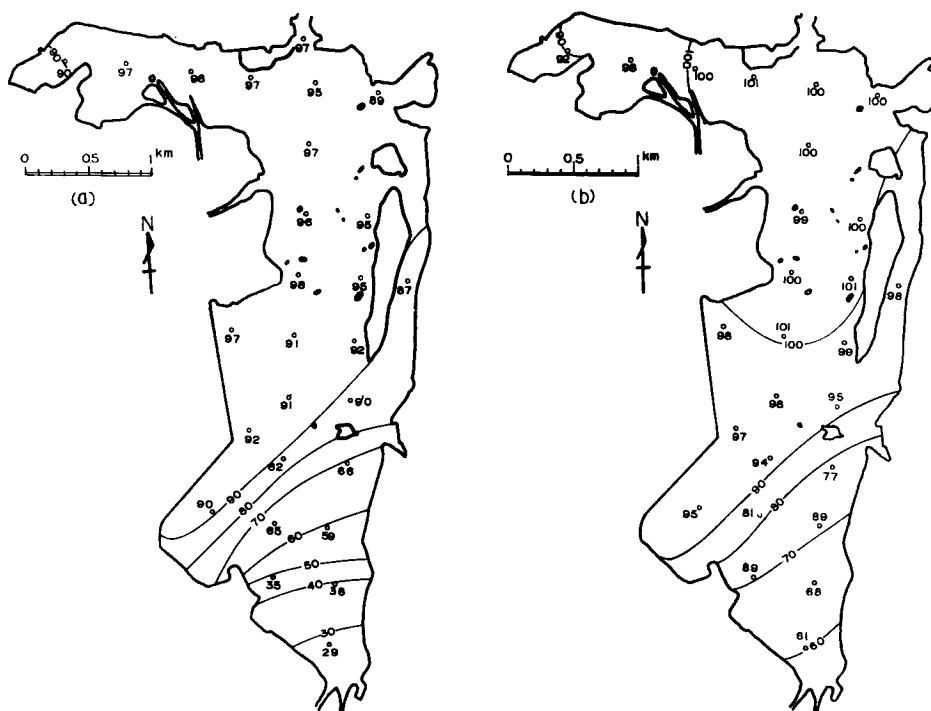
Fig. 18 Horizontal distribution of dye concentration at low water (a) and high water (b). (present state, H_1=123 cm, M.S.L.=D.L.+88 cm)
