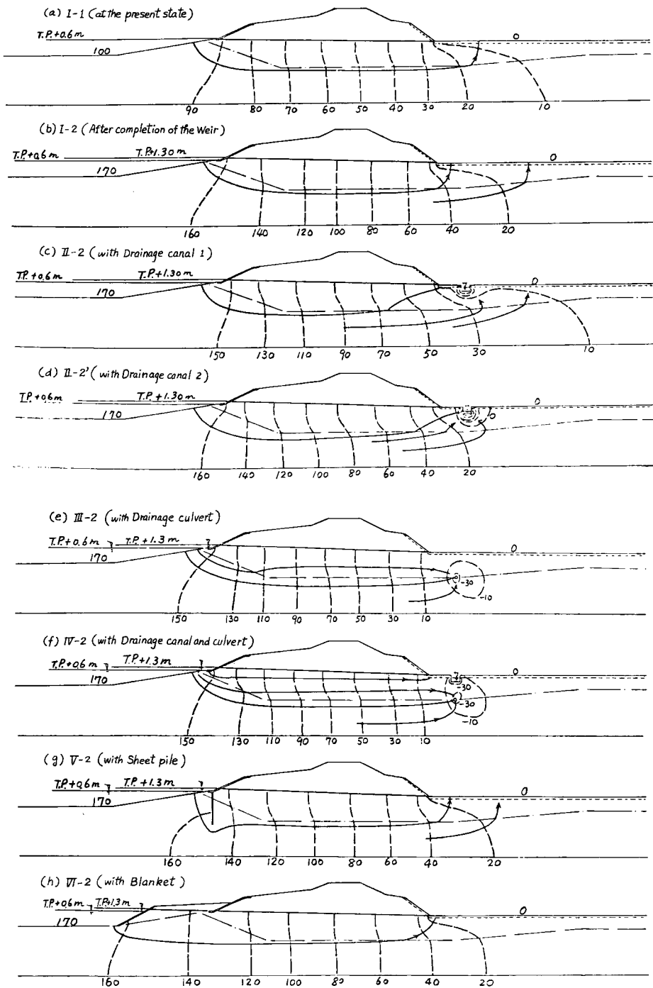
Fig. 9 Flow net.
