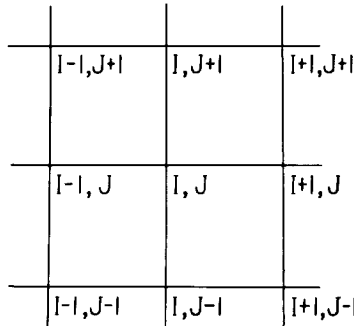
Fig. 1 Finite difference grid used to solve the differential equation.
