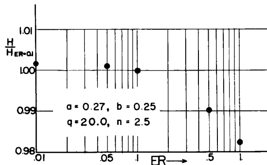
Fig. 5 Relationship between H/H_{ER=0.1} and allowable error ( ER ). H_{ER=0.1} : total water head loss calculated in ER=0.1 .
