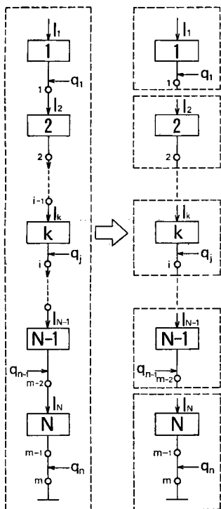
Fig. 4 Translation of an N -dimensional series type system into one-dimensional N systems by separation.
