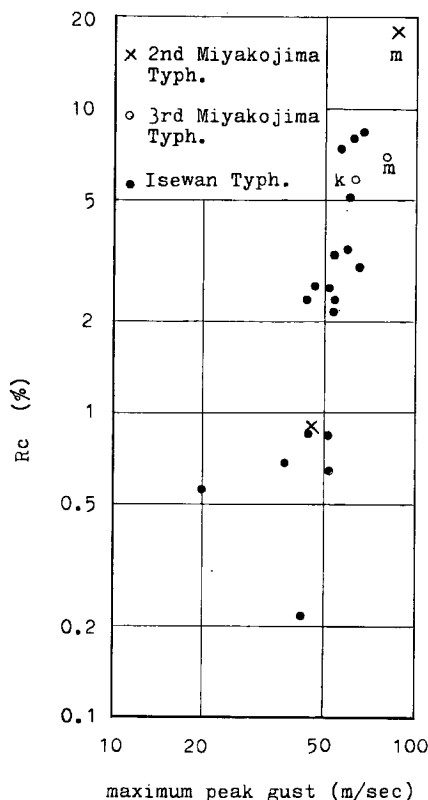
Fig. 12 Relation between rates of completely destroyed houses and maximum peak gusts. (m: Miyakojima Isl., i: Ishigakijima Isl., k: Kumejima Isl.)
