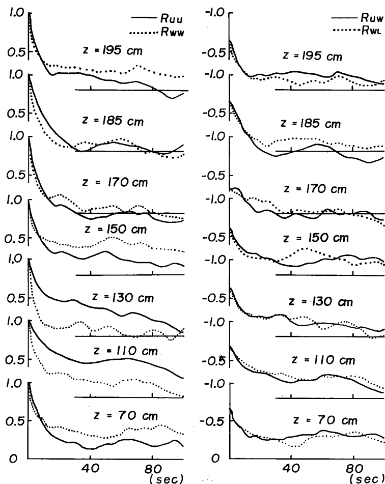
Fig. 3 Distributions of the coefficient of autocorrelation, R_{uu} , R_{wv} , and the coefficient of cross-correlation, R_{uw} , R_{uu} , in the observation A ( H = 2.1 \text{ m} ).
