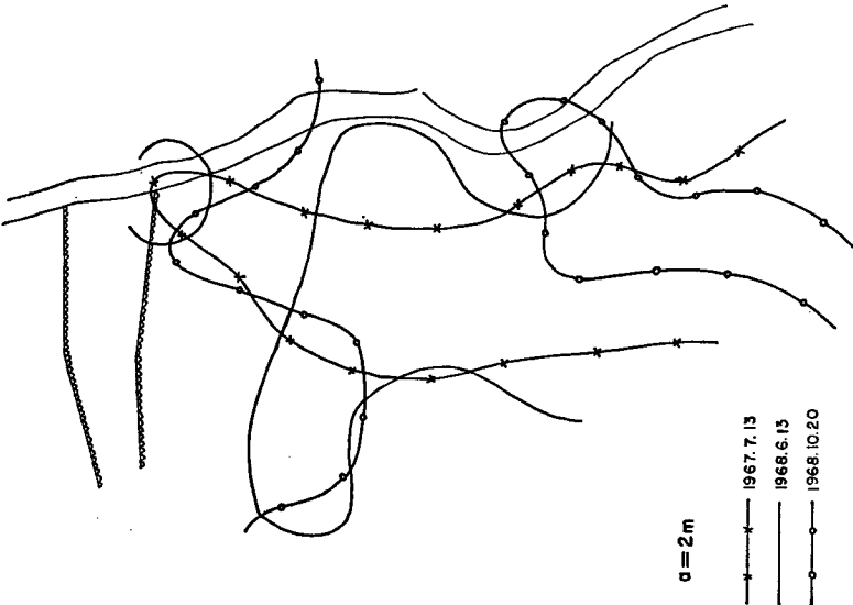
Fig. 12 The variation of the lowest apparent resistivity value during about 15 months at a=2m , Kushibayashi landslide area
