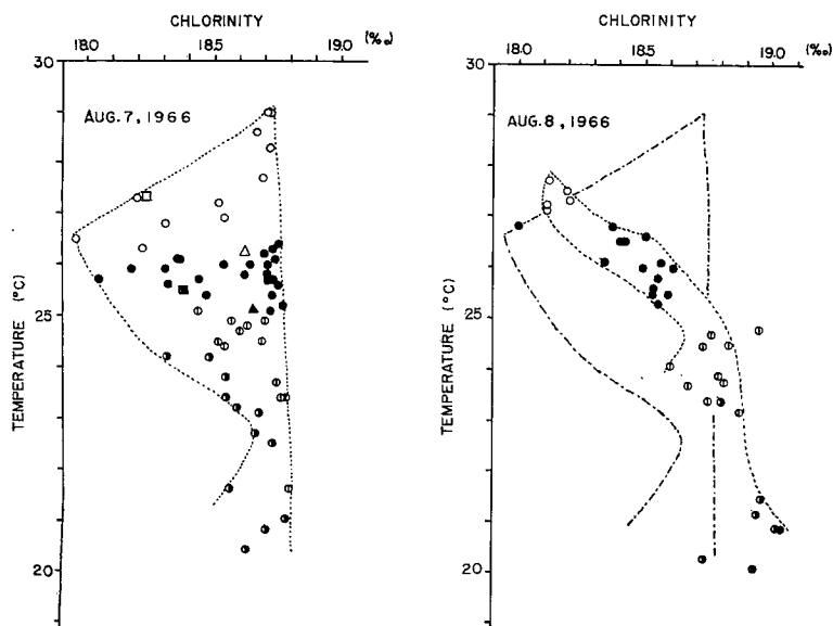
Fig. 4 T-Cl diagrams for August 7 and 8. Dash-dot line is the envelope of the T-Cl diagram of the proceeding day.
