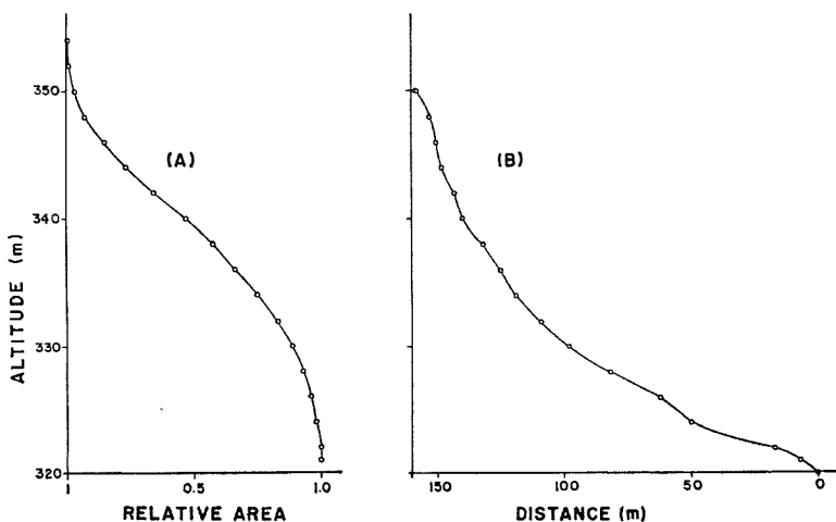
Fig. 3 The hypsometric curve (A) and the longitudinal cross section (B) of the experimental basin.
