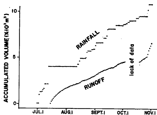
Fig. 5 Comparison of the accumulated values of rainfall and runoff.
