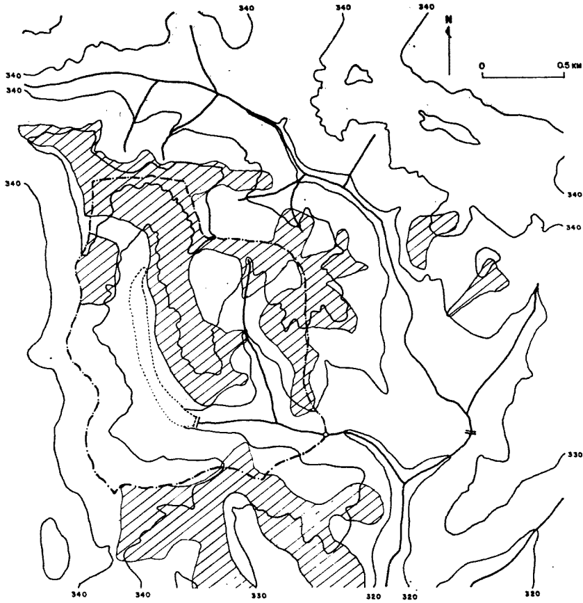
Fig. 2 A map of the Takigatani experimental basin. The bare areas (hatched part) are frequent near the ridges. — · — · — shows the devide.
