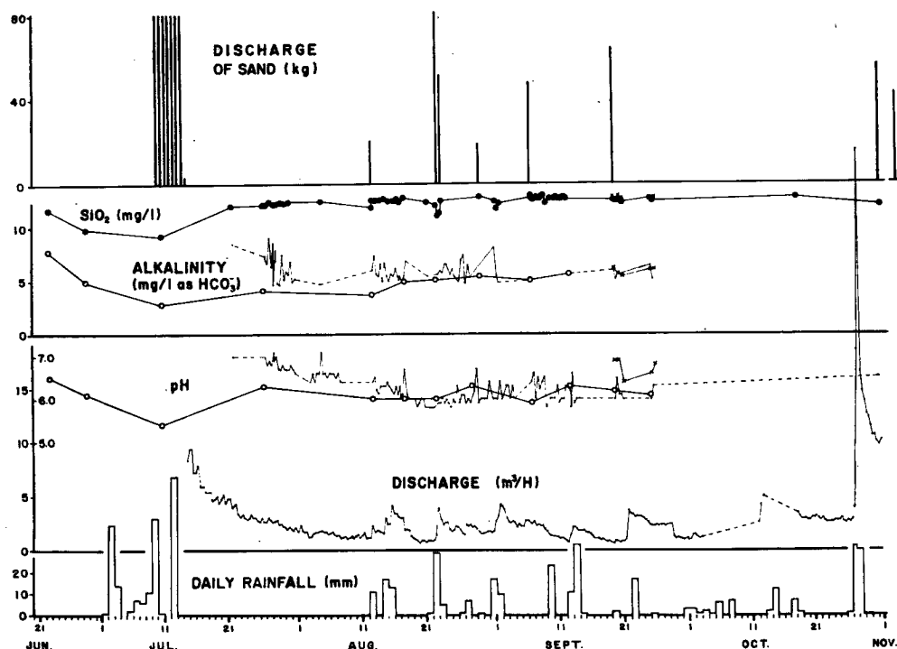
Fig. 4 Major results of the observation at the exit of the experimental basin. The chemical data shown by circles, small dots, and crosses are gotten by manual sampling, with a large automatic sampler, and with a small automatic sampler, respectively.
