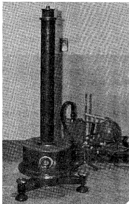
Photo. 8 Gravity variometer
