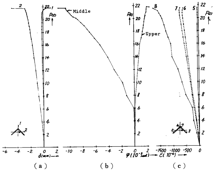
Fig. 15 Load-Deformation Relation, Series 4, \lambda=80
