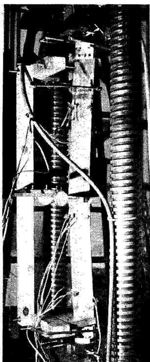
Fig. 8 Flexural Buckling (Series 2, \lambda=70 )
