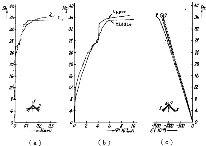
Fig. 17 Load-Deformation Relation, Series 6, \lambda=90
