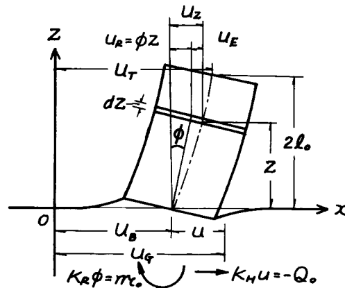
Fig. 7 Rocking of a continuous body.
