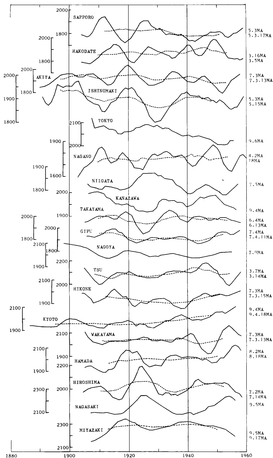
Fig. 5. T \geq 10 (full line) and T \geq 19 (dotted line) years variation in annual sum of daily amount of precipitation. Ordinate ; \log R (mm/day) \times 10^3 . Abscissa ; years. 7.3 MA ; Overlapping moving average of 7 and 3 years,
