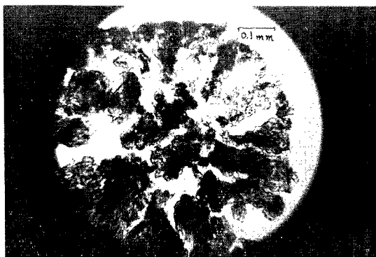
Photo. 1. Slice of prilled AN by optical microscope.
