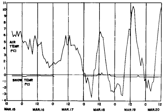
Fig. 3 The variations of temperature of the atmosphere and the snowpack. (Mar. 15 and 16 were rainy.)
