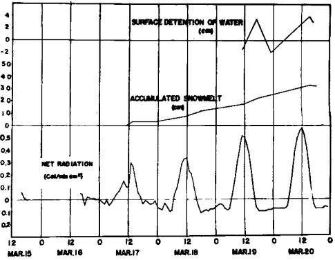
Fig. 2 Variations of the level of detained water, accumulated snowmelt, and net radiation.
