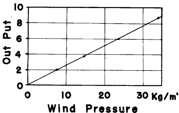
Fig. 9 Static characteristics of the pressure plate anemometer.
