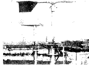
Fig. 7 New all-weather type bivane and propeller anemometer on the wind tower.
