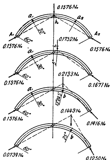
Fig. 14 The collapse of 3 hinged arch carrying a concentrated load at the distance \Delta from the centre of span ( \psi=60^\circ , h/L=0.1 )
