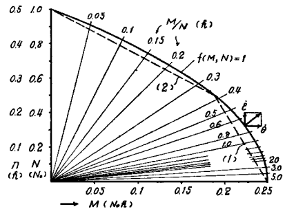
Fig. 2 The yield condition f(M, N) = 1 of rectangular section under the critical combination of bending moment M and axial force N
