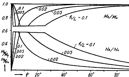
Fig. 9 M_b/M_0 , N_b/N_0 versus \psi diagrams in built-in arch carrying a concentrated load at the centre of span
