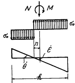
Fig. 1 The distribution of stress, rates of the axial strain and of the angle of flexure in the yield section
