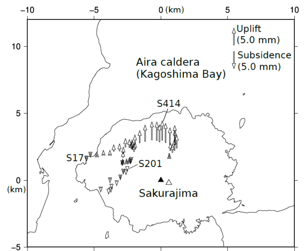
Fig. 2 Distributions of the vertical displacements of the benchmarks referred to BM.S.17 which is located at the western coast of Sakurajima during the period from November 2022 to November 2023. Solid and open triangles indicate the locations of Minamidake and Showa craters of Sakurajima volcano, respectively.
