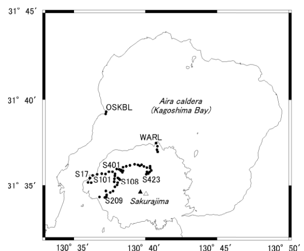
Fig. 1 Leveling benchmarks measured in the 2023 survey (solid circles). Solid and open triangles indicate the locations of Minamidake and Showa craters of Sakurajima volcano, respectively.
