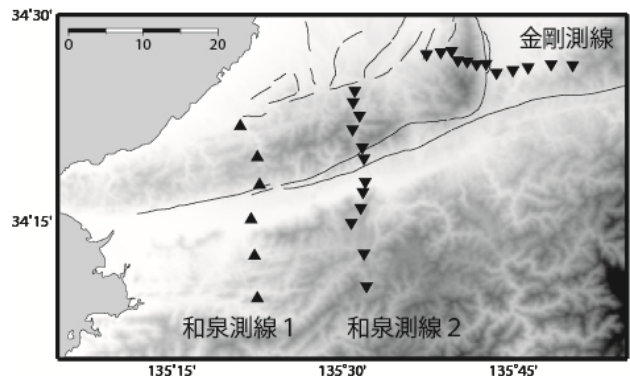
Fig.1: Magnetotelluric site locations are shown by black triangles.
