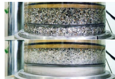
高速せん断中に発生した粒子破砕現象 Particle crushing during high-speed ring shear test
