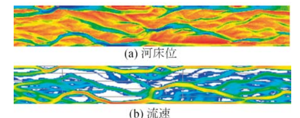
網状流路の数値解析 Numerical simulation of a braided stream
