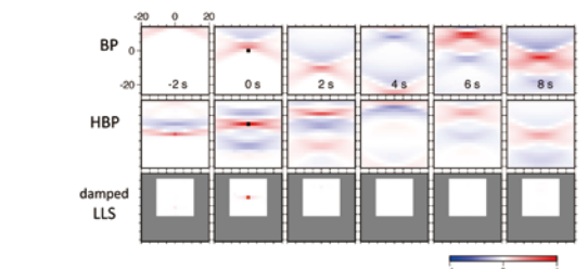
Back-Projection (BP)法、Hybrid Back-projection (HBP)法、ダンピング付き最小二乗法による点震源のイメージ。BP法、HBP法では解像度が著しく落ちていくことが分かる。Point-source images obtained by the back-projection (BP), hybrid back-projection (HBP), and damped least-square solution. The image of the point source, put at the origin, cannot be well reproduced by the BP and HBP methods.
