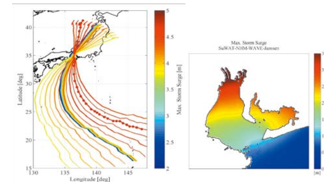
伊勢湾に襲撃する台風の経路と高潮水位の関係 Simulated typhoon courses and storm surges modeled from the Isewan typhoon
