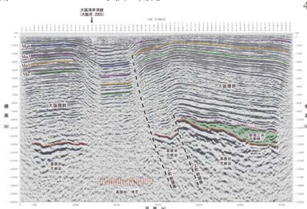
上町断層帯南部における反射法地震探査（堺-高石測線）結果と構造解釈 Geologic interpretation of the depth section by a seismic reflection survey across the Uemachi fault system
