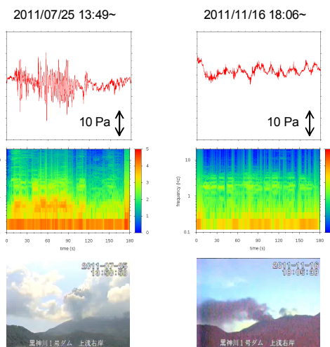
Fig. 2 Three minutes waveforms of infrasound and their spectrograms on 25 July (13:49) and 16 Nov. (18:06), respectively. Eruption images are also displayed.
