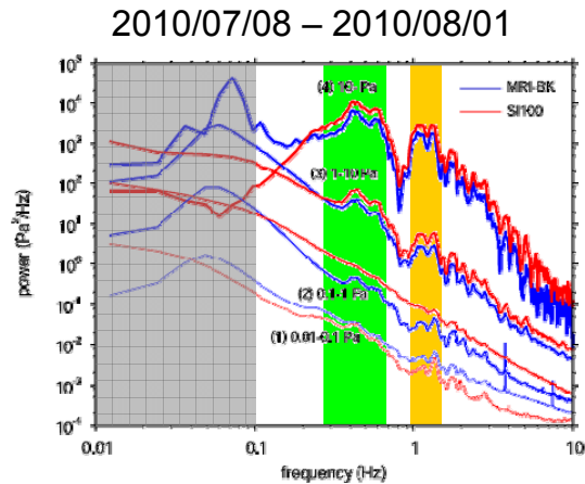
Fig. 4 Power spectrums of Sakurajima infrasound records with RMS amplitudes observed at the Seto station of JMA.
