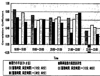
Fig. 14 Correlation coefficient above the points where there is no surface observation.
