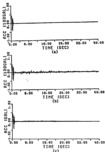
Fig. 10 Medium impulse response (interstation distance: 100m).
