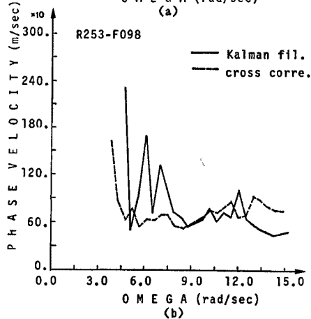
Fig. 18 (a) Comparison of dispersion curves (R253-F089). (b) Comparison of dispersion curves (R253-F098).
