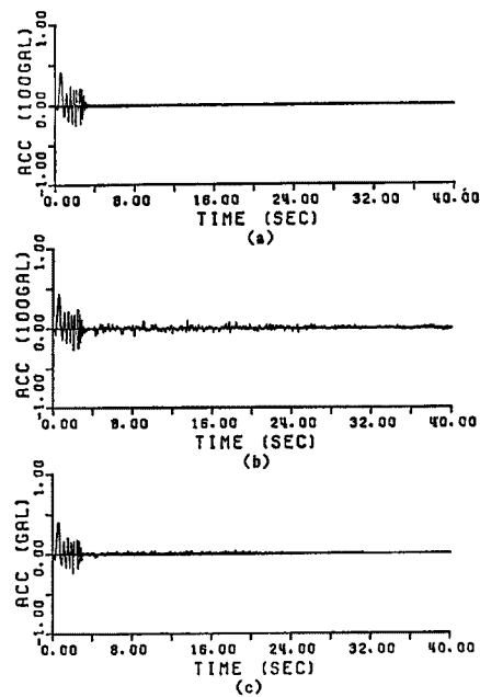
Fig. 11 Medium impulse response (interstation distance: 300m).
