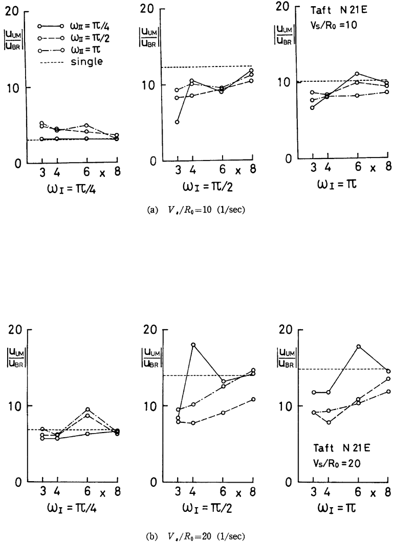
Fig. 20 Maximum responses of upper mass against separation distance. Taft N21E, d=2 , e=1 .
