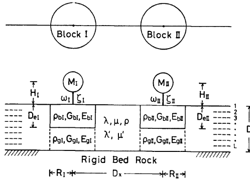
Fig. 3 Two-structures-soil system.
