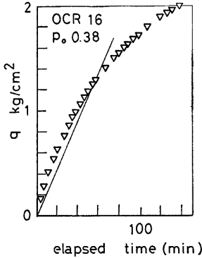
Fig. 20. Shear stress rate under strain controlled CU test for O.C.R. 16, p_0 = 0.38 \text{ kg/cm}^2 .
