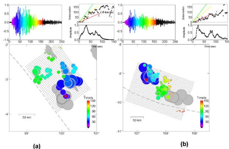
Figure 1. (a) 2010 Sumatra earthquake. Top show the seismograms recorded at station HMNH, the stacked amplitude curve and rupture velocity. The red, yellow and green lines present a rupture velocity of 1.0, 2.0, and 3.0 km/s, respectively. Bottom shows the locations, timing and amplitudes of the maximum amplitudes for the high frequency band. Red star shows the epicenter. The gray solid circles indicate the low frequency centroids. (b) Same results for the 2006 Java tsunami earthquake.
