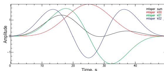
Figure 1 4\pi prolate eigentapers
