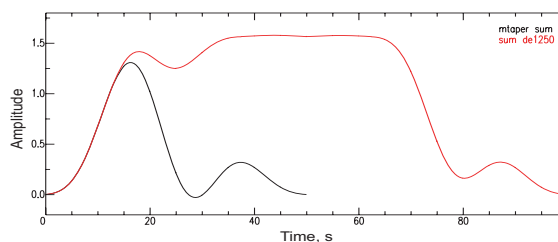
Figure 2 Extended-time multi-taper
